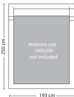
Paola bed IV - top view
